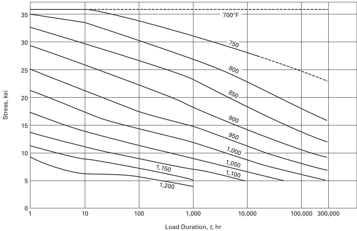
Figure E-100.5-4 S_t — Allowable Stress Intensity Values, ksi, 2\frac{1}{4}\text{Cr-1Mo}
