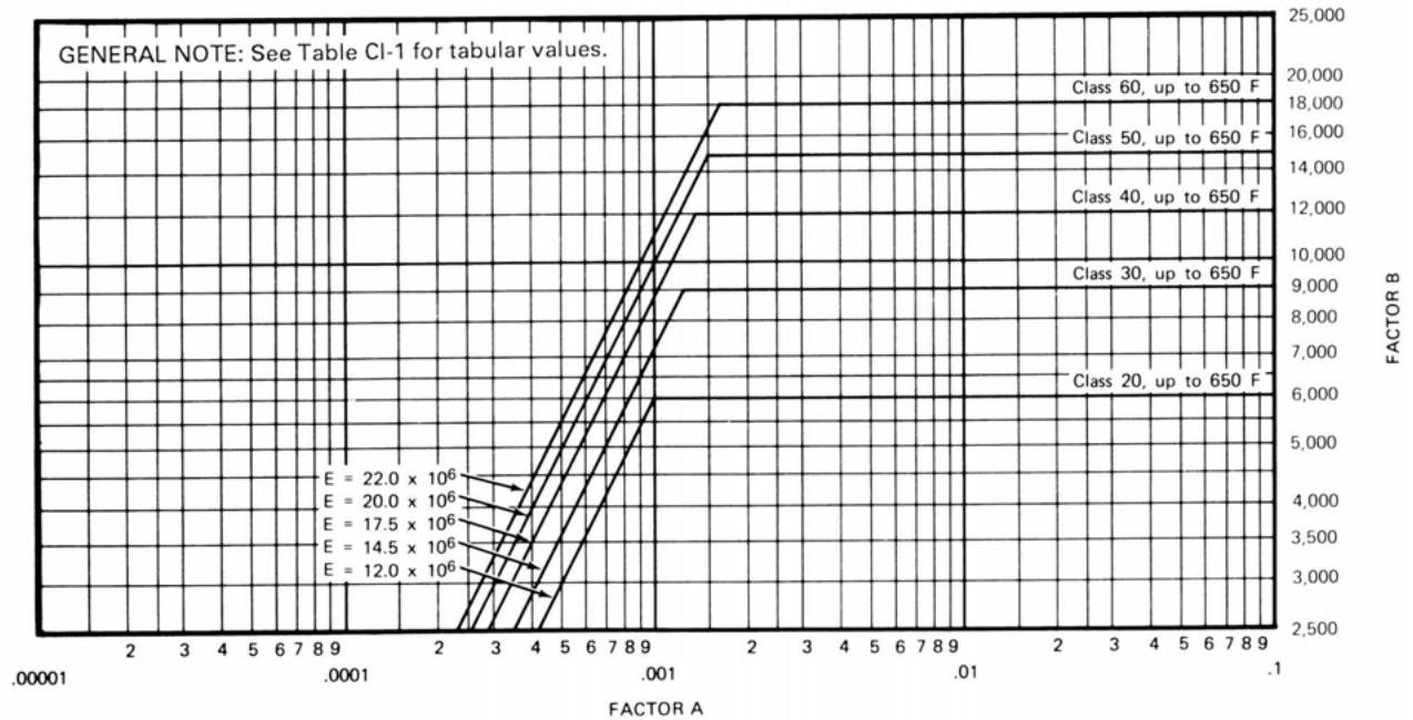
Figure CI-1 Chart for Determining Shell Thickness of Components Under External Pressure Developed for Cast Iron
