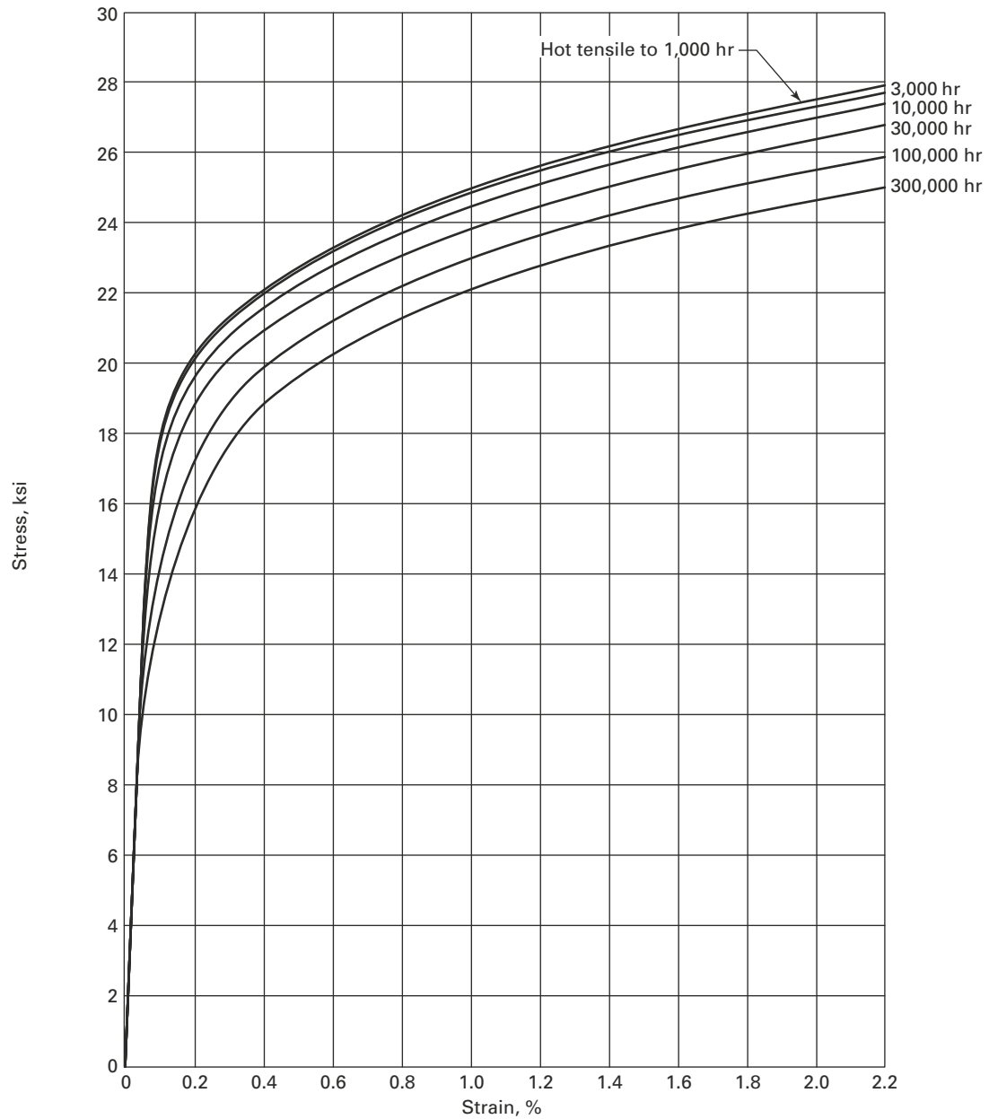
Figure E-100.19-4 Average Isochronous Stress-Strain Curves for Type 316 SS at 950°F
