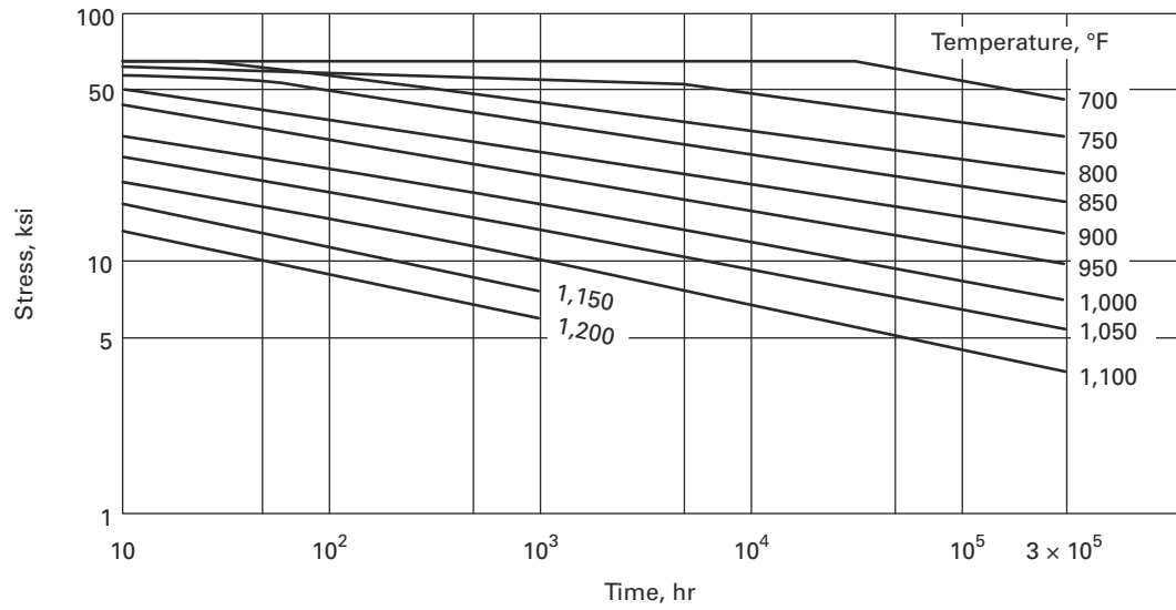
Figure E-100.7-4 Expected Minimum Stress-to-Rupture Values, ksi, 2 \frac{1}{4} Cr-1Mo
