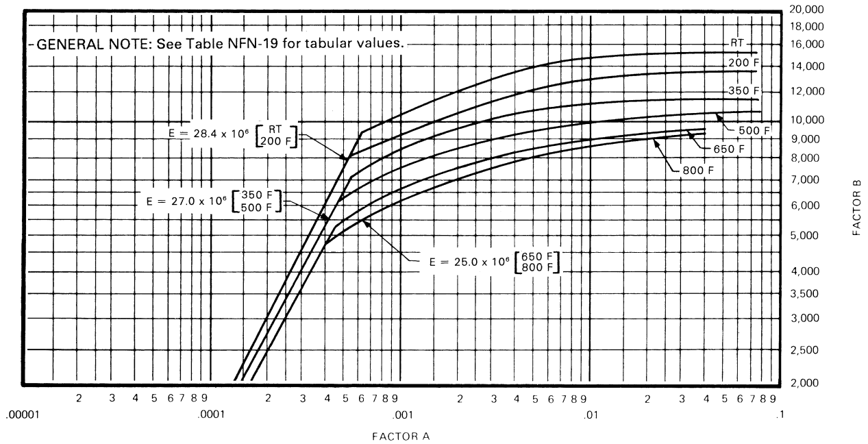
Figure NFN-19 Chart for Determining Shell Thickness of Components Under External Pressure Developed for Nickel–Molybdenum–Chromium–Iron–Copper Alloy N06985 Having a Minimum Yield Strength of 30 ksi
