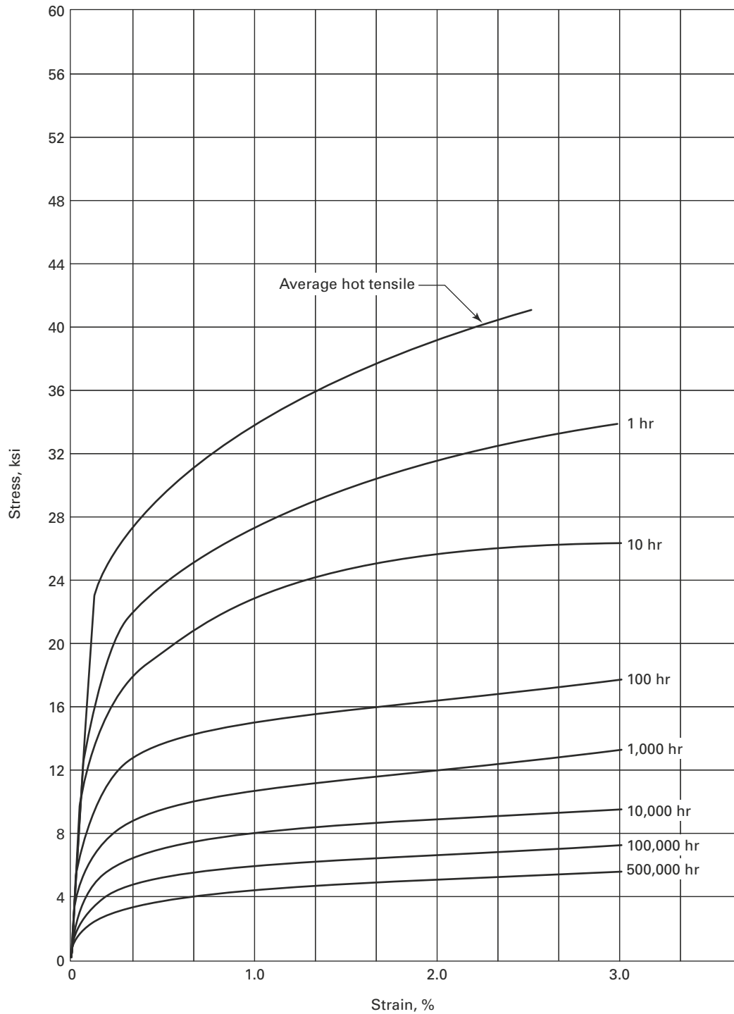
Figure E-100.21-8 Average Isochronous Stress-Strain Curves for Annealed 2\frac{1}{4}\text{Cr}-1\text{Mo} at 1,050^\circ\text{F}
