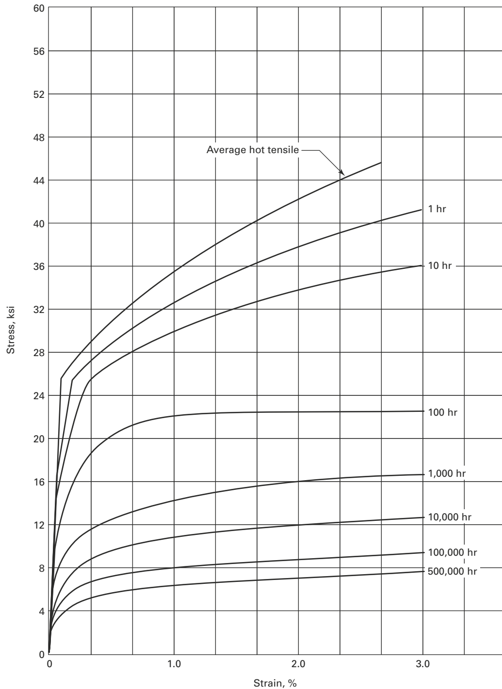
Figure E-100.21-7 Average Isochronous Stress-Strain Curves for Annealed 2\frac{1}{4}\text{Cr}-1\text{Mo} at 1,000^\circ\text{F}
