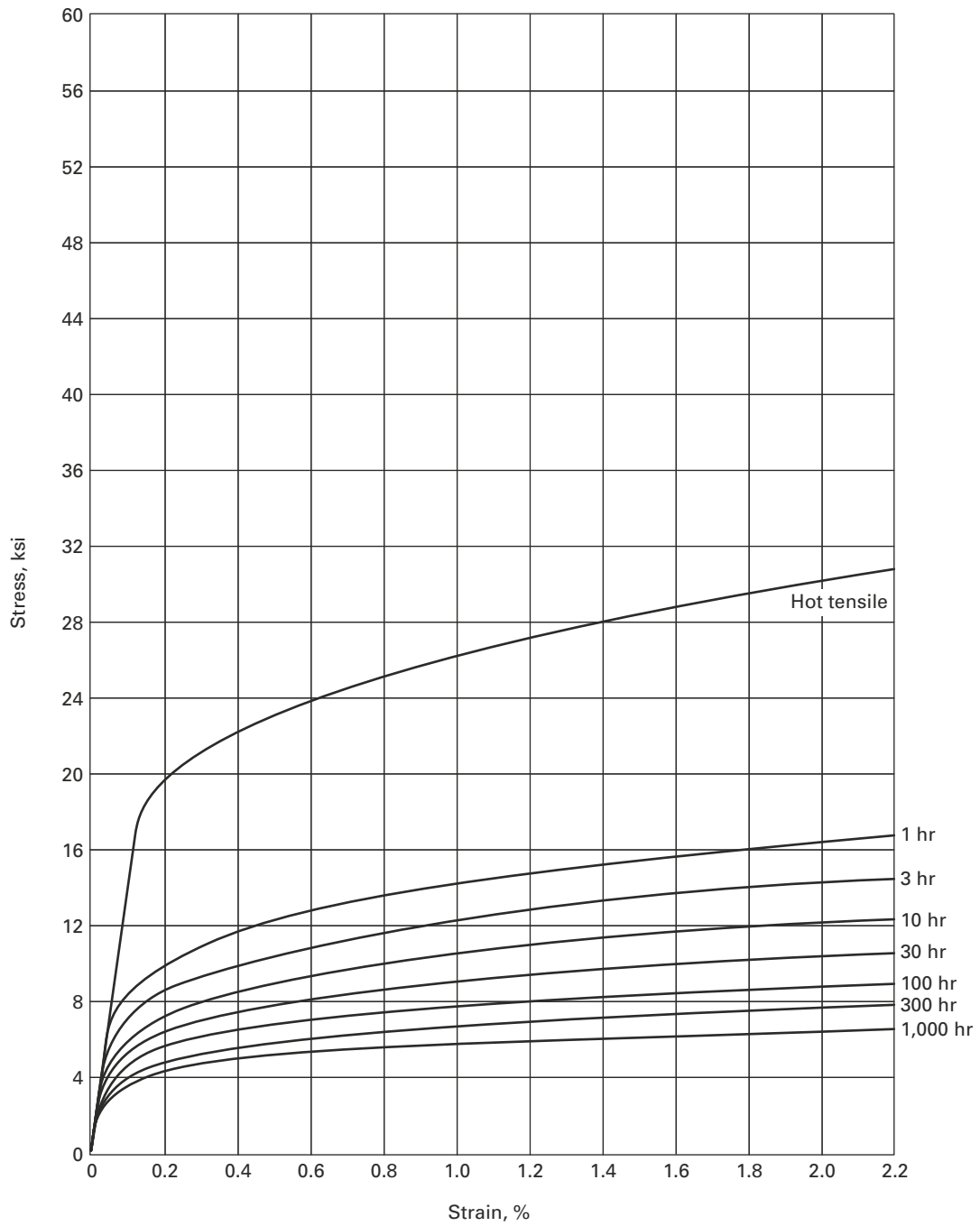
Figure E-100.21-11 Average Isochronous Stress–Strain Curves for Annealed 2\frac{1}{4}\text{Cr} –1Mo at 1,200°F
