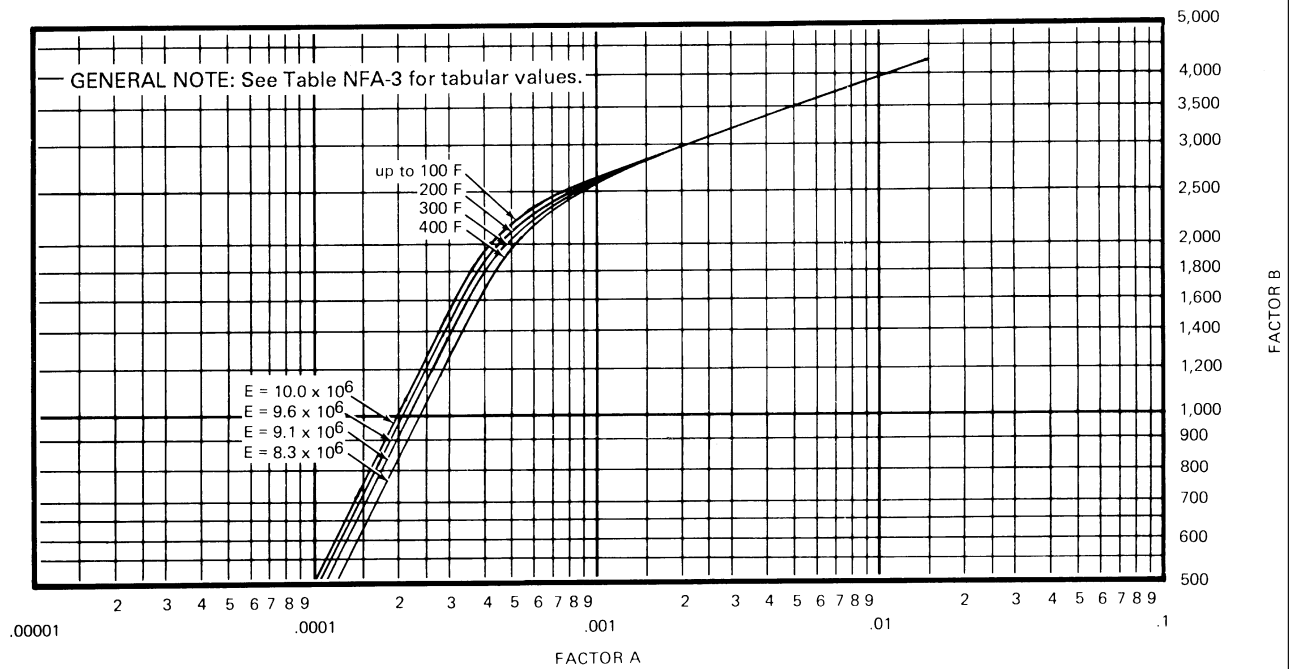
Figure NFA-3 Chart for Determining Shell Thickness of Components Under External Pressure Developed for Aluminum Alloy 3004 in 0 Temper
