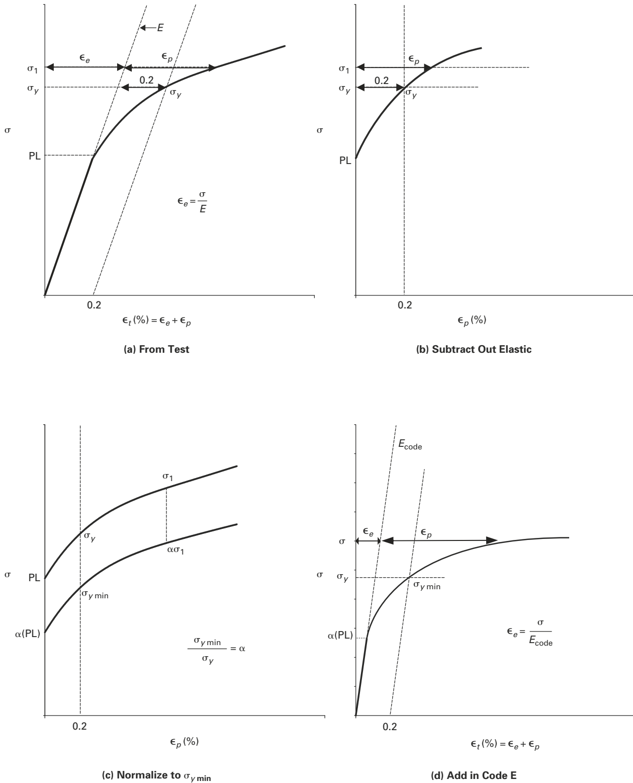
Figure 3-700.1 Normalization of Test \sigma - \epsilon to \sigma_{ymin} and E_{code}
