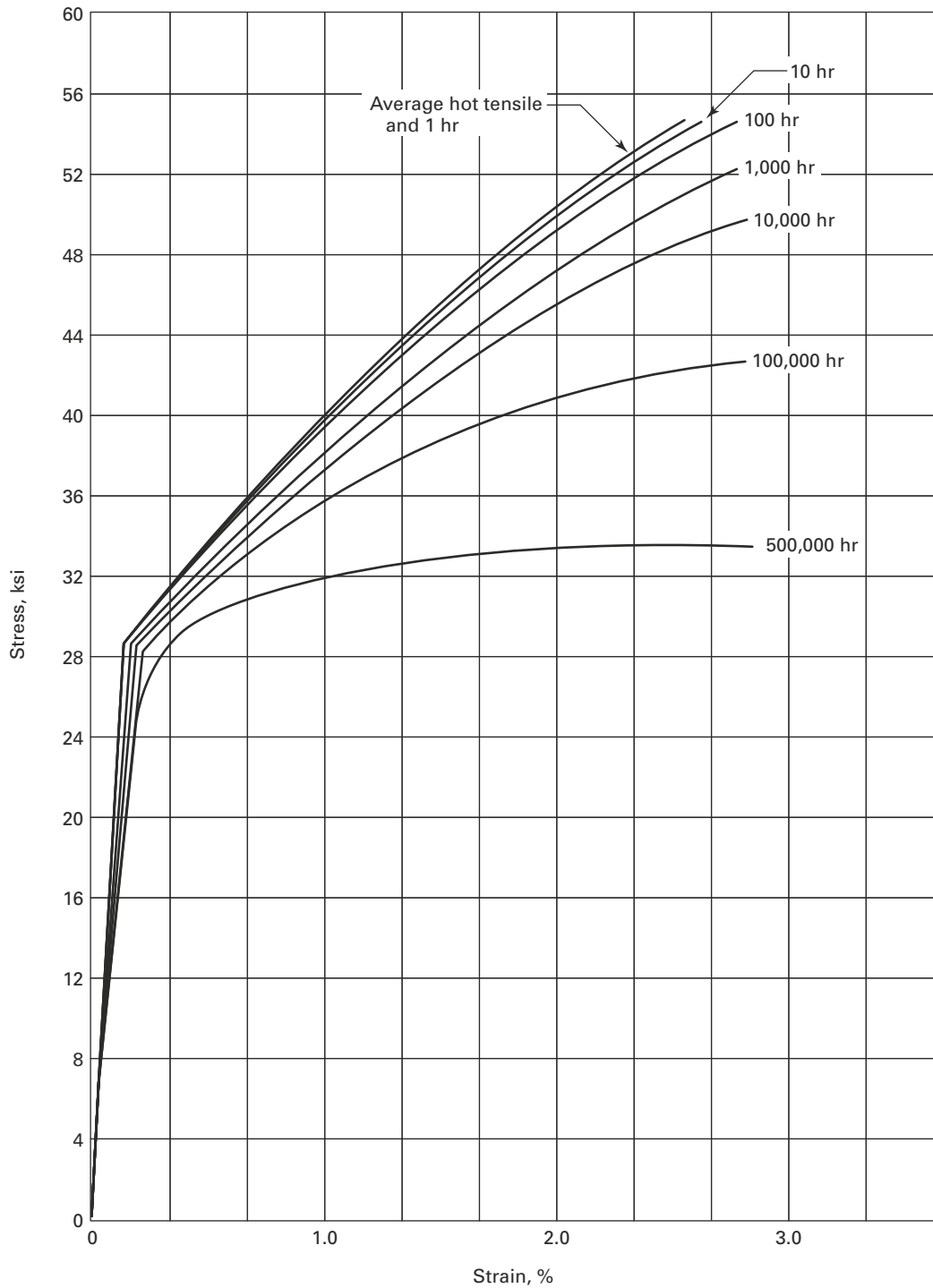
Figure E-100.21-2 Average Isochronous Stress-Strain Curves for Annealed 2\frac{1}{4}\text{Cr}-1\text{Mo} at 750°F
