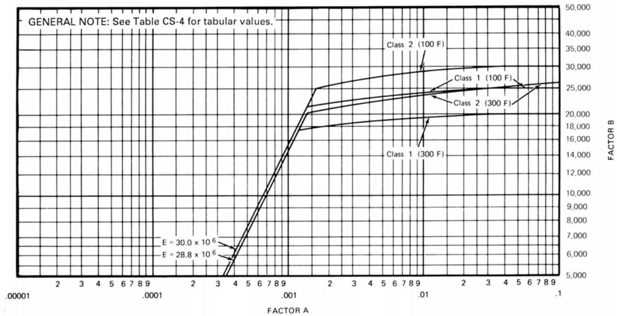
Figure CS-4 Chart for Determining Shell Thickness of Components Under External Pressure Developed for SA-537 Thickness 2\frac{1}{2} in. and Less
