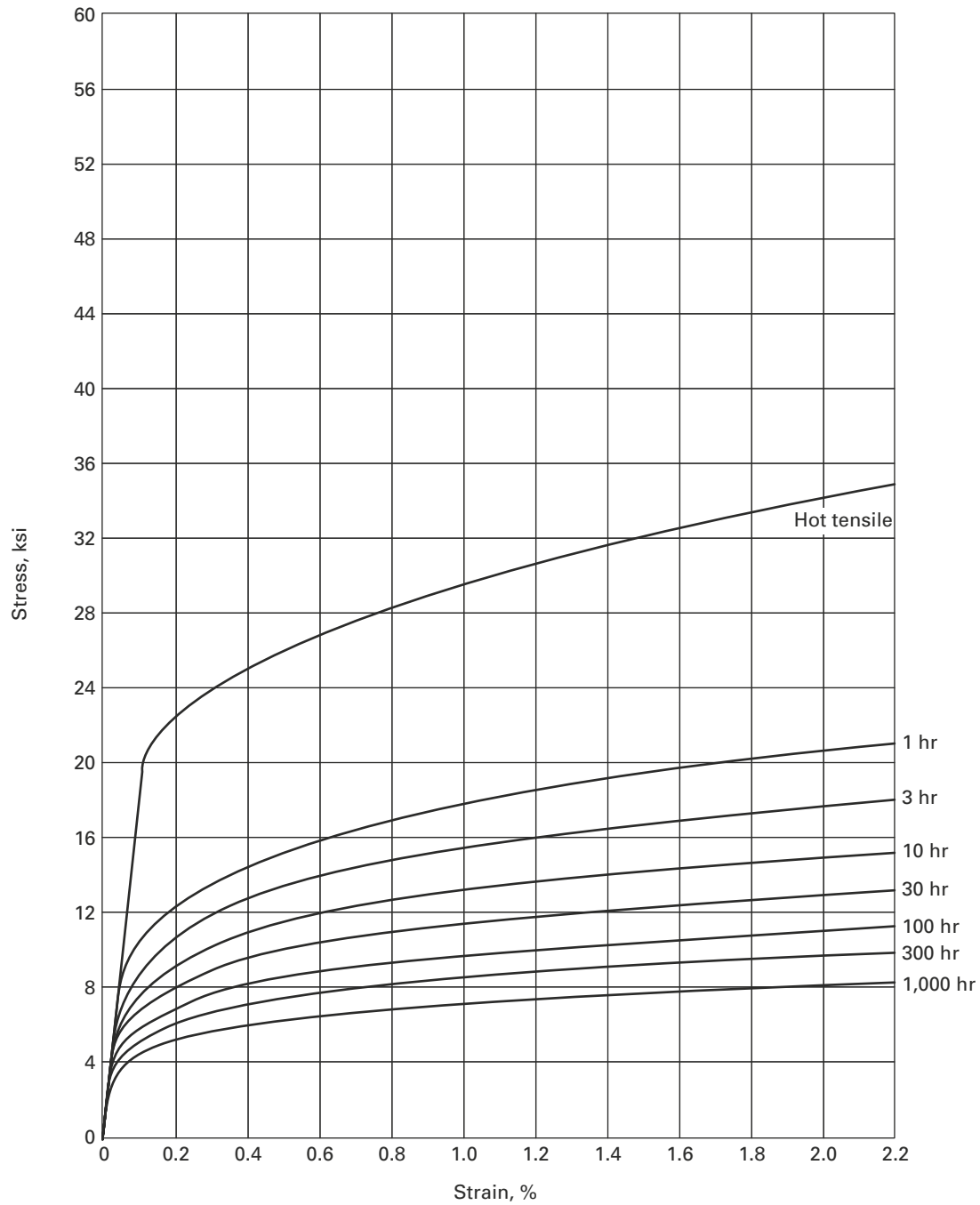
Figure E-100.21-10 Average Isochronous Stress-Strain Curves for Annealed 2\frac{1}{4} Cr-1Mo at 1,150°F
