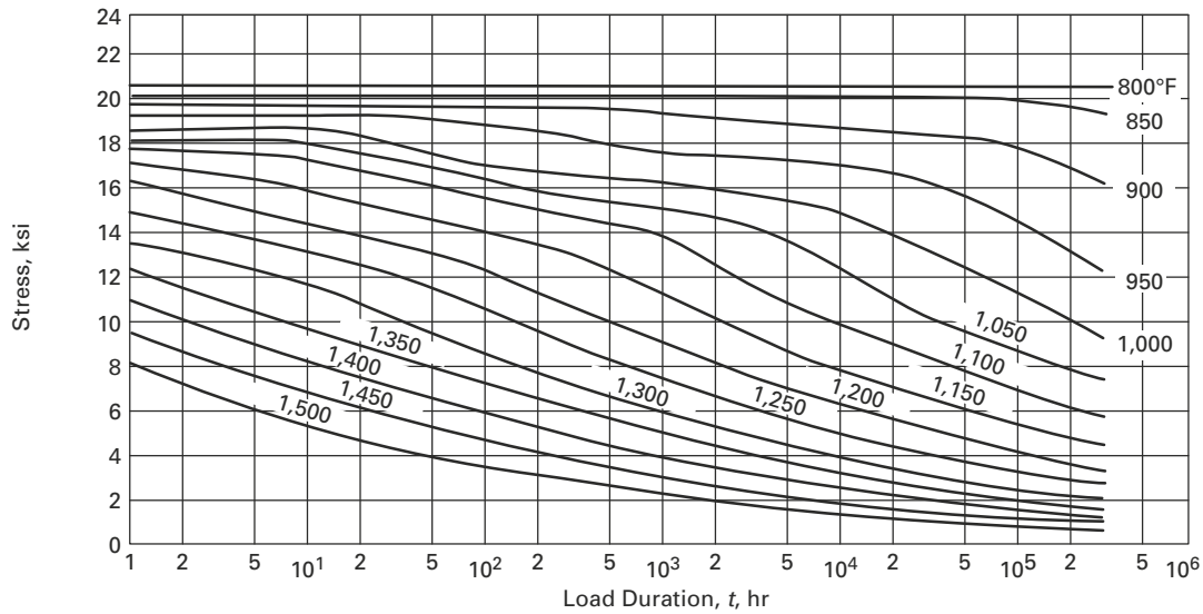
Figure E-100.5-1 S_t — Allowable Stress Intensity Values, ksi, Type 304 SS
