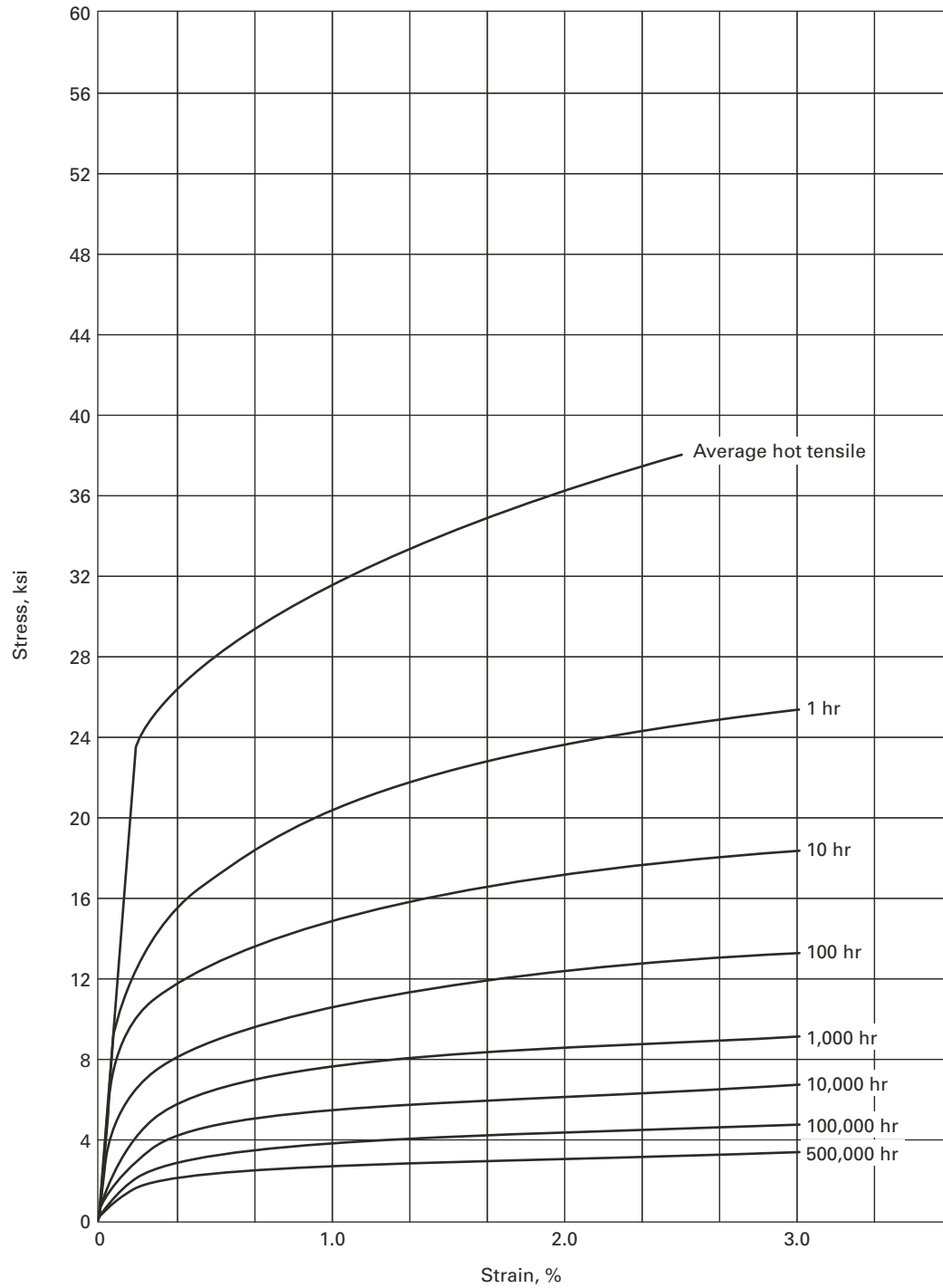
Figure E-100.21-9 Average Isochronous Stress–Strain Curves for Annealed 2\frac{1}{4} Cr–1Mo at 1,100°F
