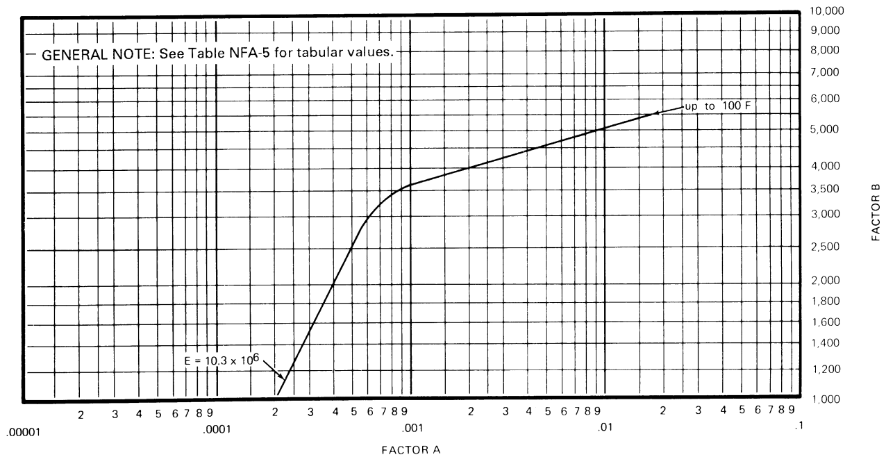
Figure NFA-5 Chart for Determining Shell Thickness of Components Under External Pressure Developed for Aluminum Alloy 5154 in 0 Temper
