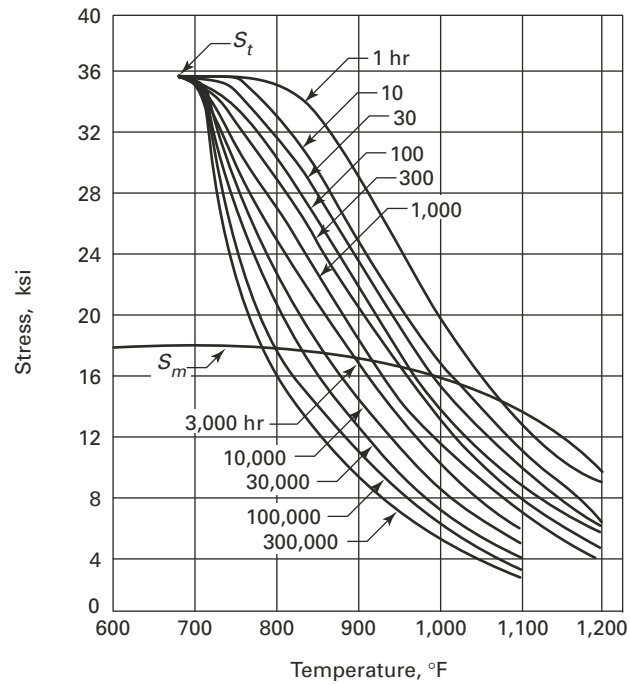
Figure E-100.4-4 S_{mt} — Allowable Stress Intensity Values, ksi, 2\frac{1}{4}\text{Cr}-1\text{Mo}
